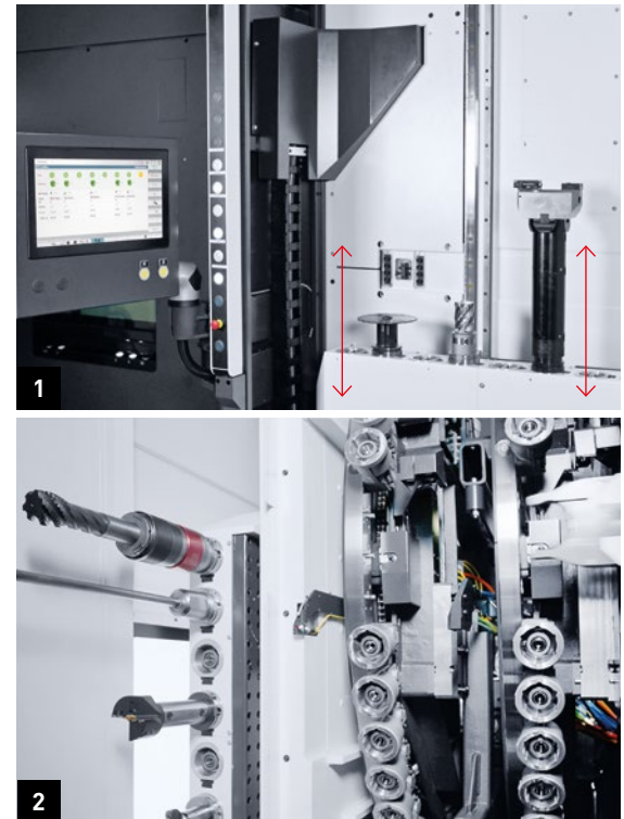
1. Perfect ergonomics: Height-adjustable tool loading station for setting up sets of 8 tools each weighing 30 kg incl. tool identification. 2. Automatic exchanging of the tools from the loading station to the wheel magazine.
