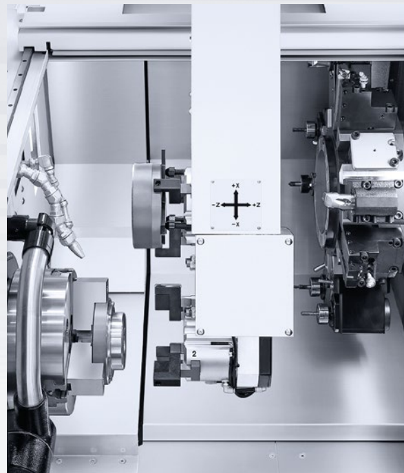
Loading arm with integrated double gripper for workpieces up to ø200 mm, 150 mm in length and 15 kg (per hand).
