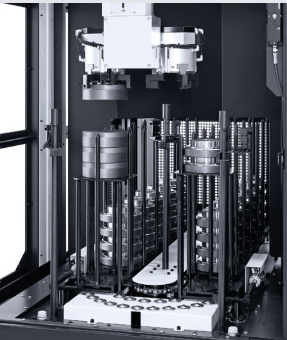
Storage for up to 20 pallets with a maximum weight of 75 kg and up to 26 to a maximum of 35 kg per station.
